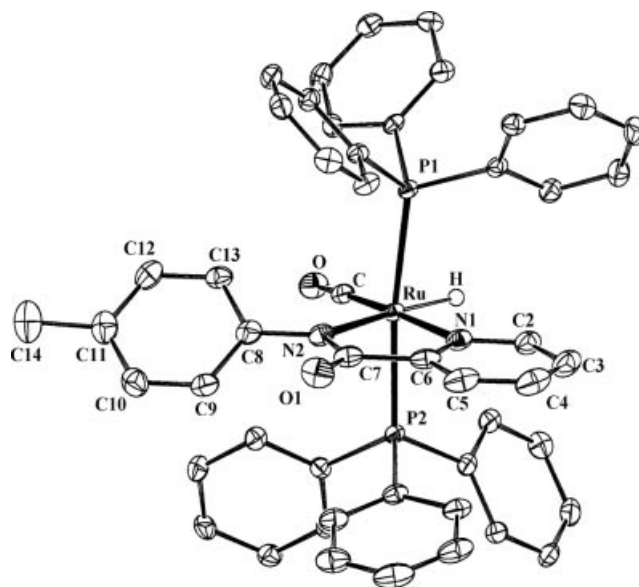
Figure 3. View of the 2-CH 3 complex.
