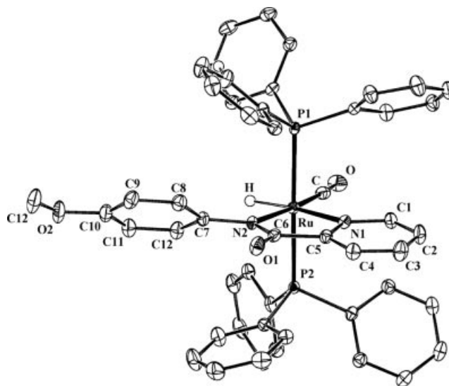
Figure 1. View of the 1-OCH 3 complex.
