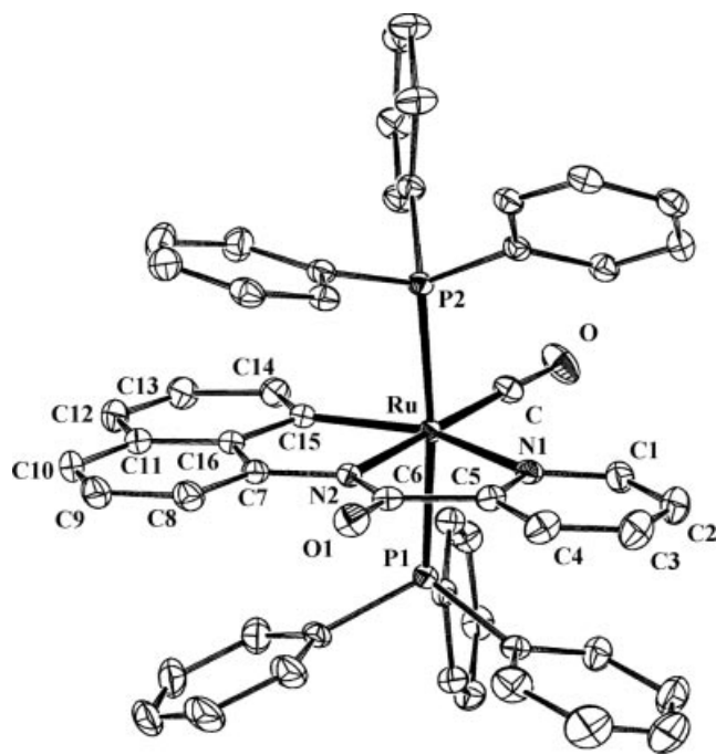
Figure 4. View of complex 3.
