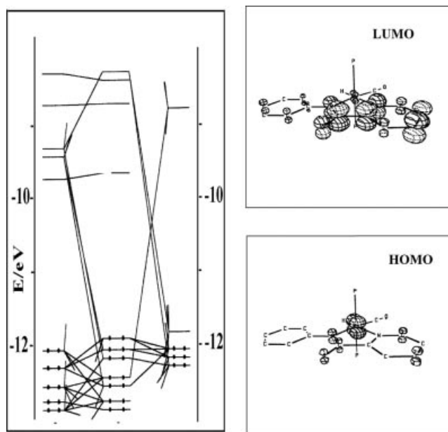
Figure 5. Partial molecular orbital diagram of the 1-H complex.
